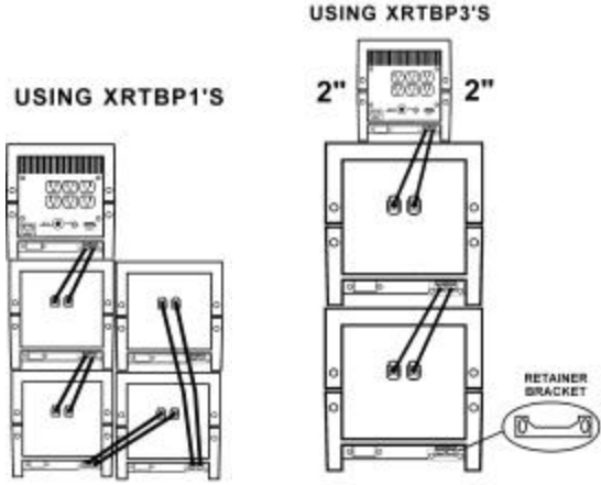
Battery Pack Connection Diagram
